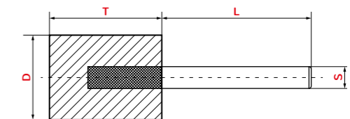
MOUNTED POINT
