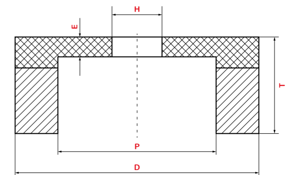
CUP WHEEL WITH PLATE
